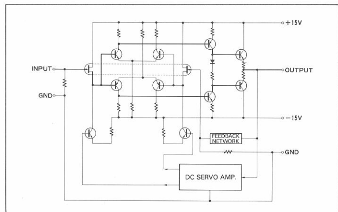
(FIG. 2) SERVO CONTROLLED HIGH-LEVEL AMP.
